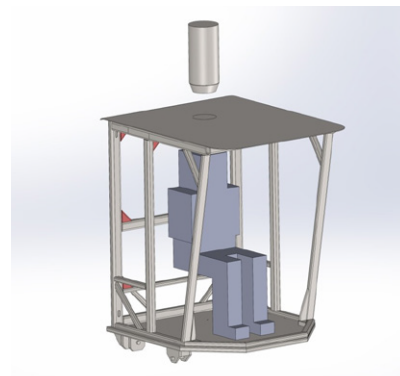
Fig. 12. FOPS simulation loads
