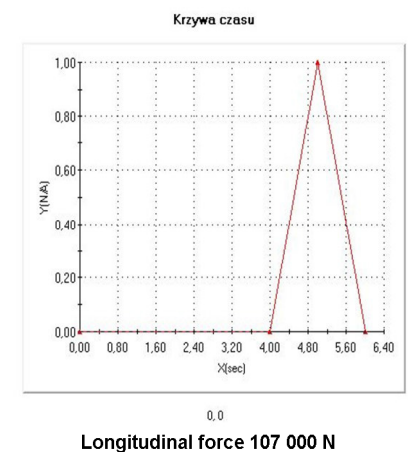
Fig. 16. ROPS load force coefficients vs time and force values
