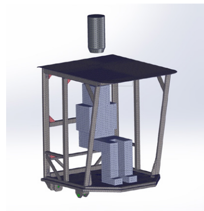
Fig. 11. Structure mesh
